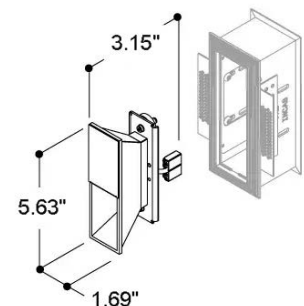
Fixture Dimensions
