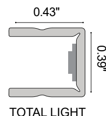
Fixture Dimensions
