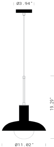
Fixture Dimensions
