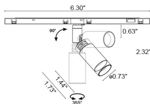
Fixture Dimensions
