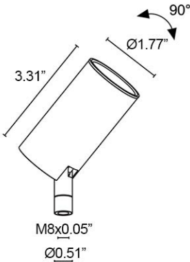
Fixture Dimensions
