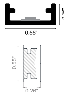
Fixture Dimensions
