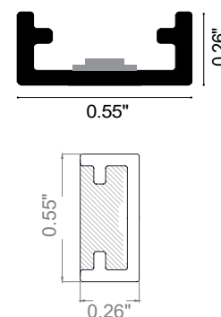
Fixture Dimensions
