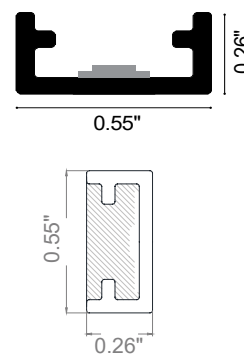
Fixture Dimensions
