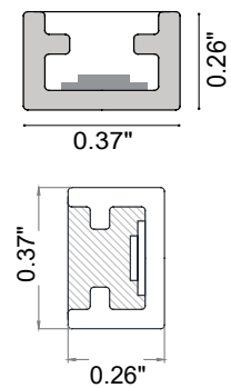
Fixture Dimensions
