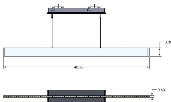
Fixture Dimensions
