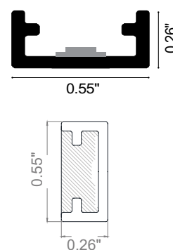
Fixture Dimensions
