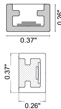
Fixture Dimensions
