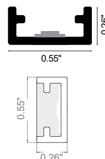
Fixture Dimensions
