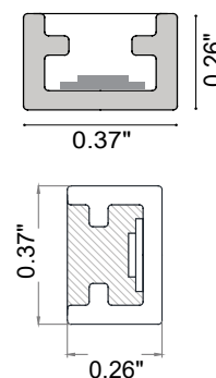
Fixture Dimensions
