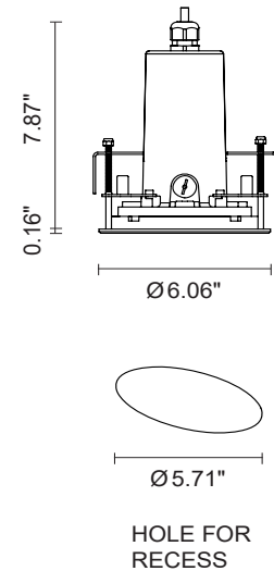
Fixture Dimensions
