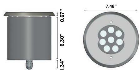
Fixture Dimensions
