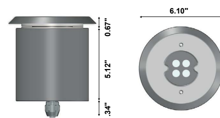
Fixture Dimensions
