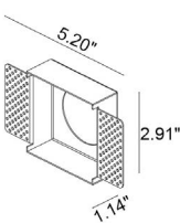
WCA28 Outer Casing For Plasterboard
