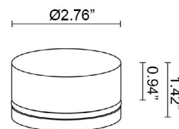
Fixture Dimensions
