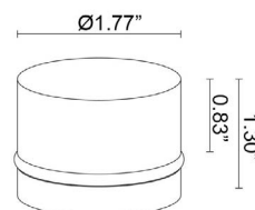
Fixture Dimensions
