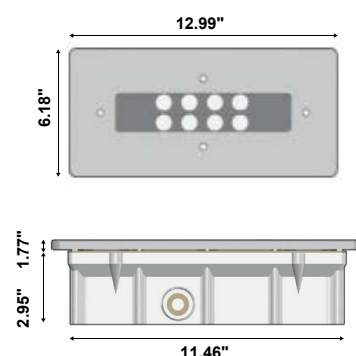
Fixture Dimensions
