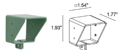
WBA09__ Asymmetric Snoot For Snoots include one of the below finishes: E - White F - Gray H - Anthracite T - Cor-ten 5 - Jasper Green C - Custom RAL
