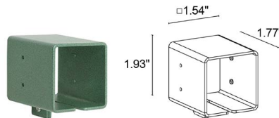
WBA08__ Standard Snoot For Snoots include one of the below finishes: E - White F - Gray H - Anthracite T - Cor-ten 5 - Jasper Green C - Custom RAL
