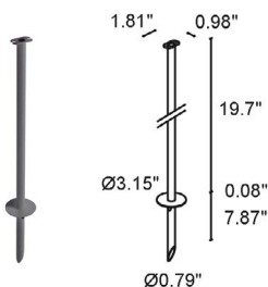
WP1006__ (Length 19.69") WP1007__ (Length 31.50") Ground Spike with Bracket Include one of the below finishes: E - White H - Anthracite T - Cor-ten 5 - Jasper Green C - Custom RAL
