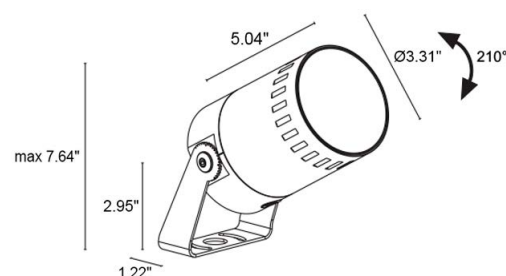
Fixture Dimensions
