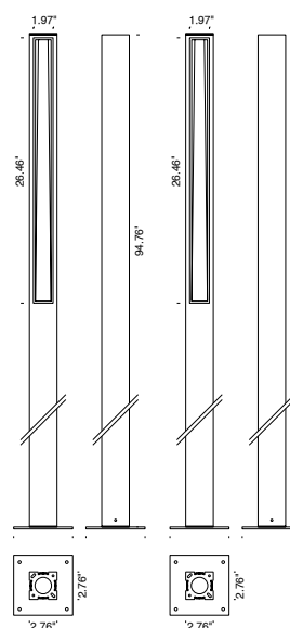
Fixture Dimensions
