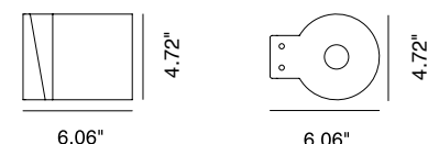
Fixture Dimensions
