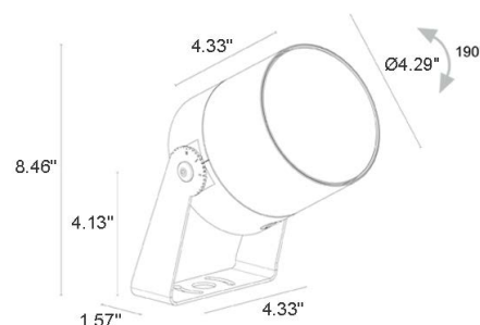
Fixture Dimensions
