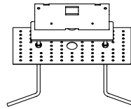
PT65000 Flange Kit with 4 Anchor Bolts 9.06" w x 10.63" h (REQUIRED)
