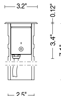
Fixture Dimensions
