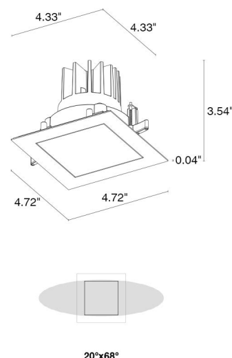
Fixture Dimensions
