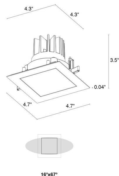
Fixture Dimensions
