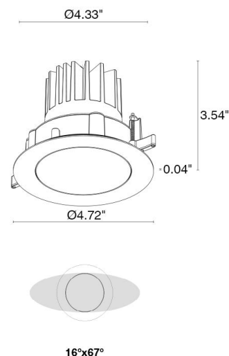
Fixture Dimensions
