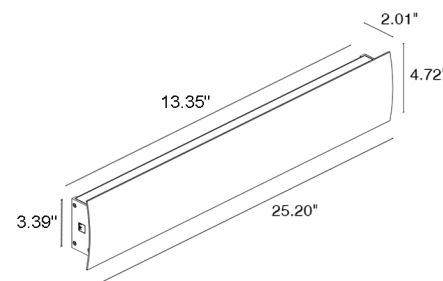
Fixture Dimensions
