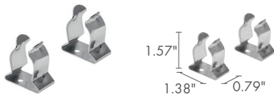
WM0501 Clips Pair
