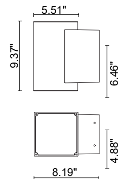
Fixture Dimensions
