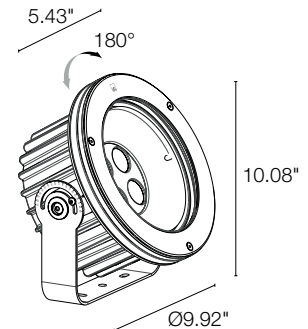
Fixture Dimensions
