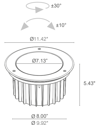
Fixture Dimensions
