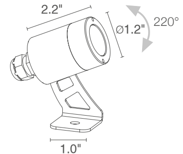
Fixture Dimensions
