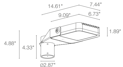
Fixture Dimensions
