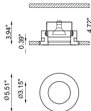
Fixture Dimensions
