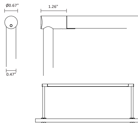
Fixture Dimensions
