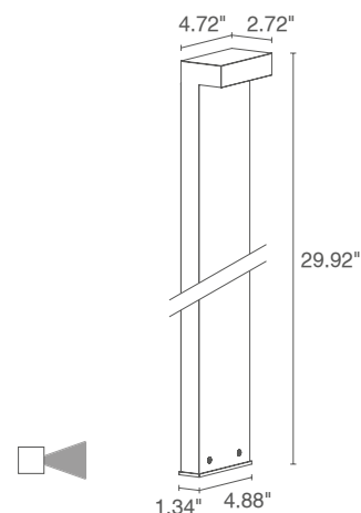
Fixture Dimensions
