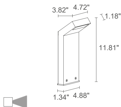
Fixture Dimensions
