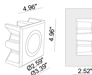
Wall Cut-Out: 5.20" x 5.20" Fixture Dimensions
