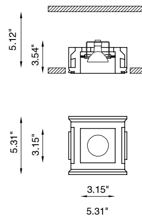
Fixture Dimensions
