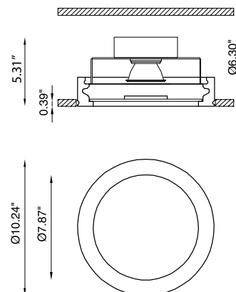
Fixture Dimensions
