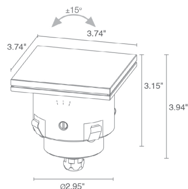
Fixture Dimensions
