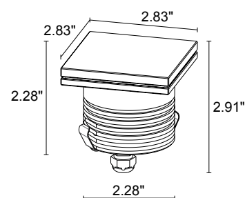
Fixture Dimensions
