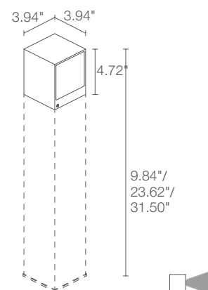
Fixture Dimensions
