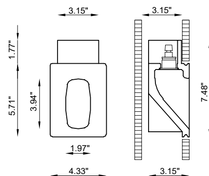
Fixture Dimensions
