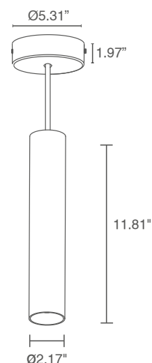
Fixture Dimensions
